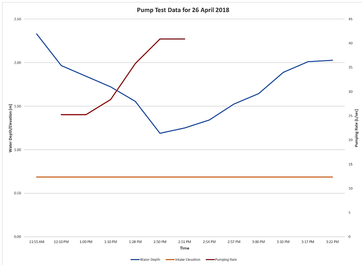
Figure 2 Pump Test Data for 26 April 2018
