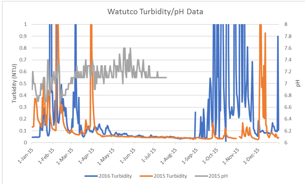
Figure 17 Raw Water Quality Data
