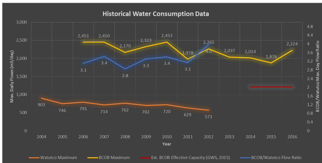
Figure 14 Watutco and BCOB Maximum Daily Water Consumption Data
