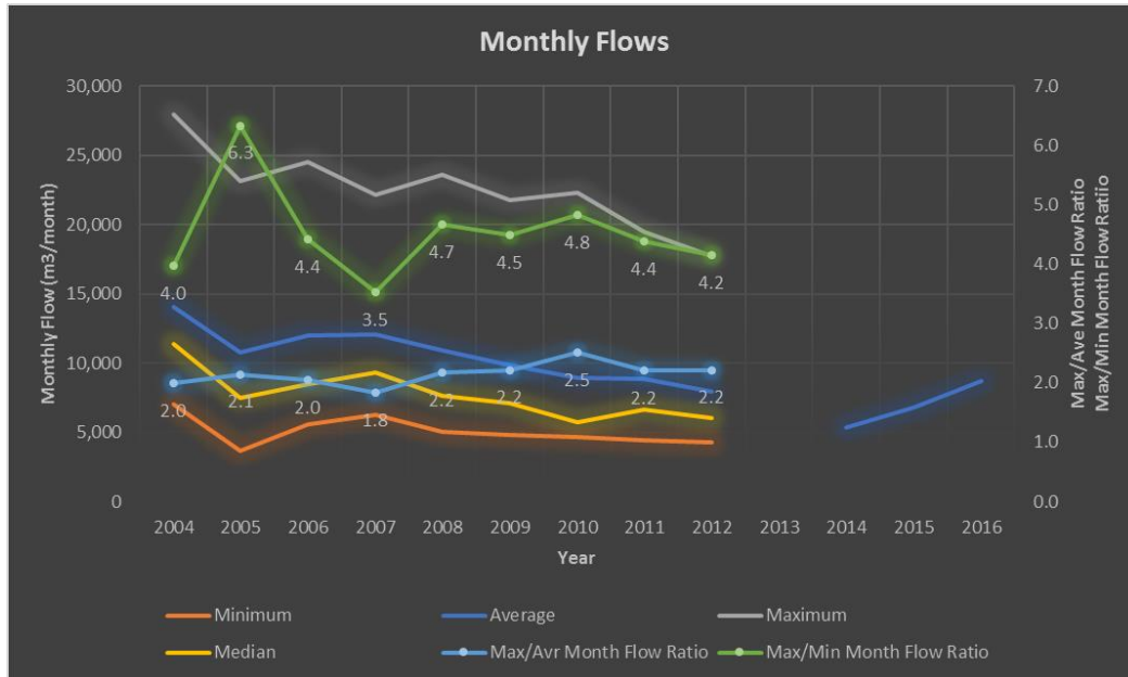
Figure 9 Monthly Flow Data (2004-2012)
