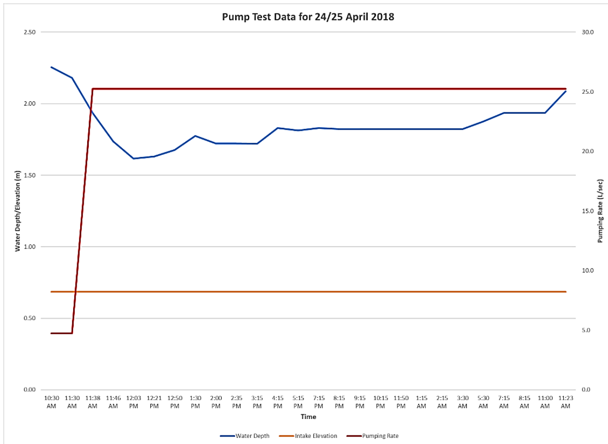
Figure 1 Pump Test Data for 24/25 April 2018
