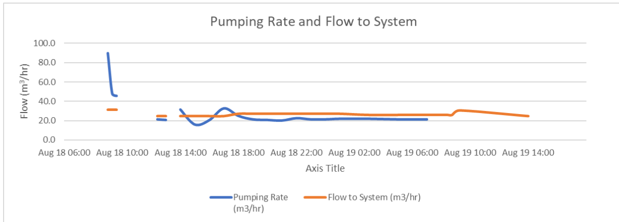
Figure 3 Pump Test Data for 18/19 August 2018
