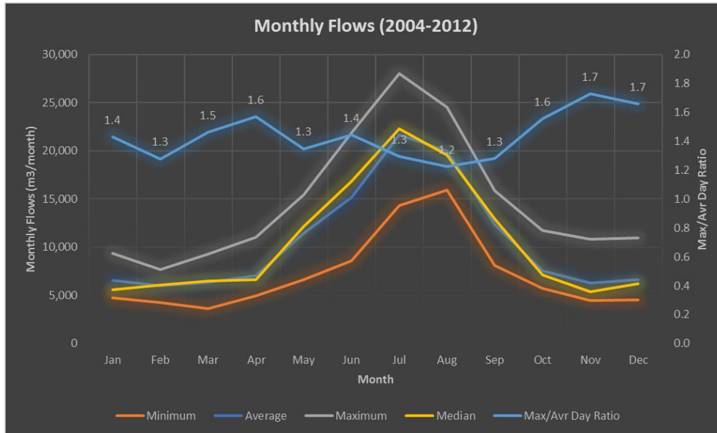
Figure 8 Monthly Flows (2004-2012)
