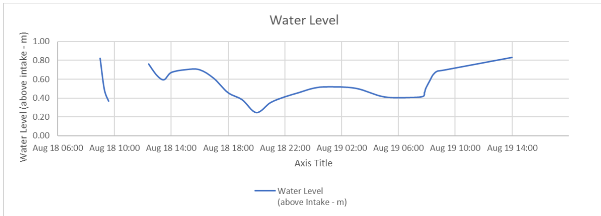
Figure 4 Pump Test Data for 18/19 August 2018
