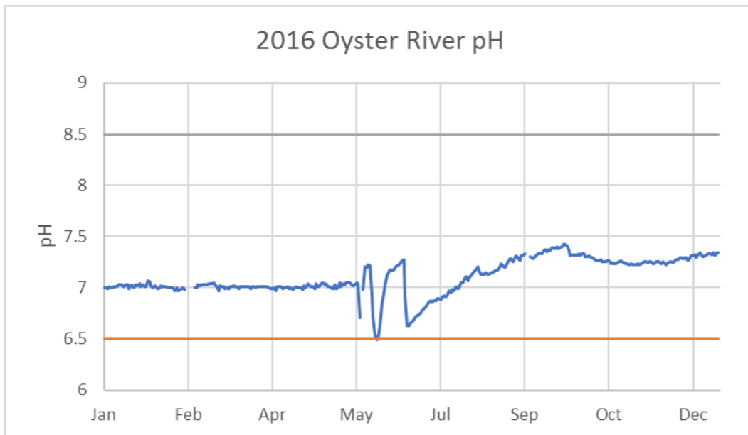
Figure 20 2016 Oyster River pH Data
