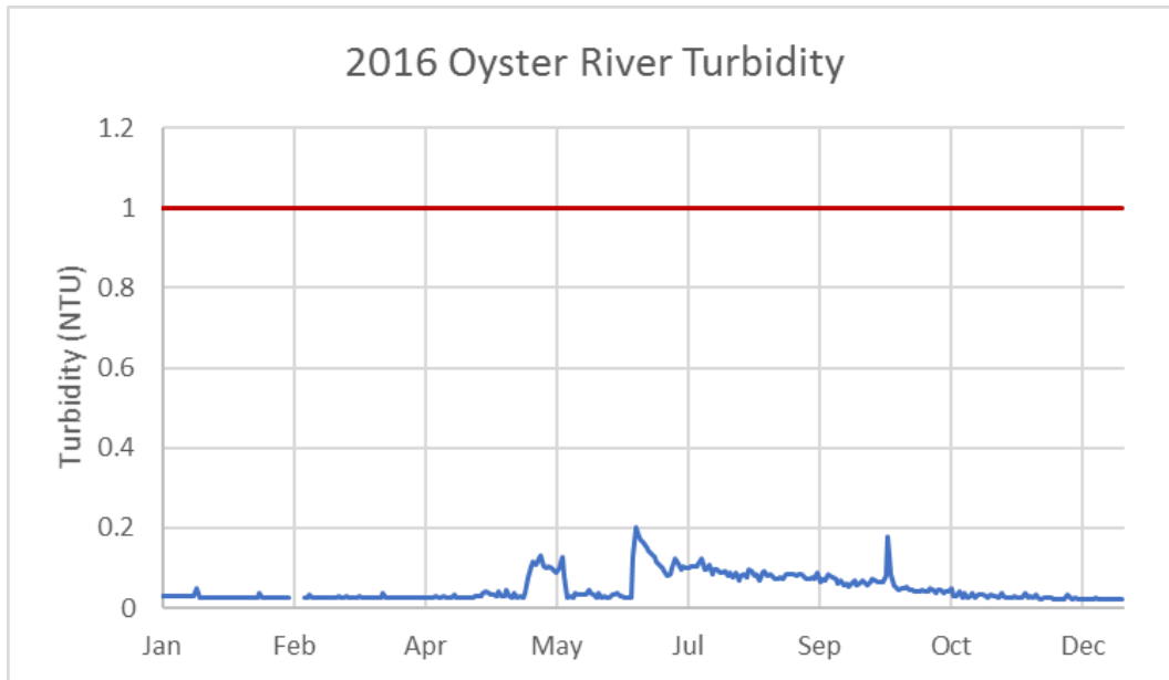
Figure 19 2016 Oyster River Turbidity Data
