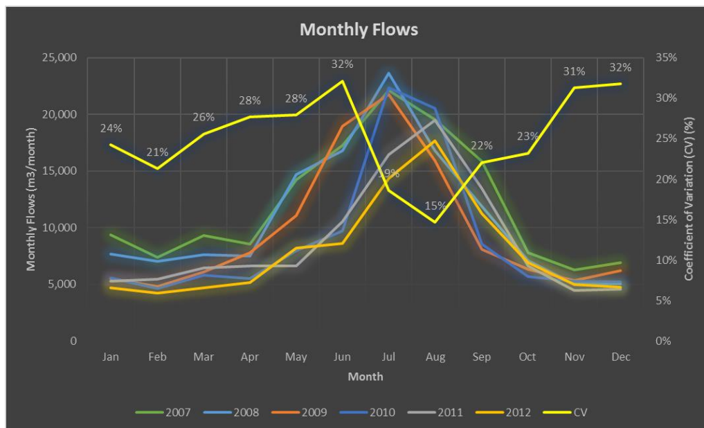
Figure 7 Monthly Flow Distributions (2007-2012)
