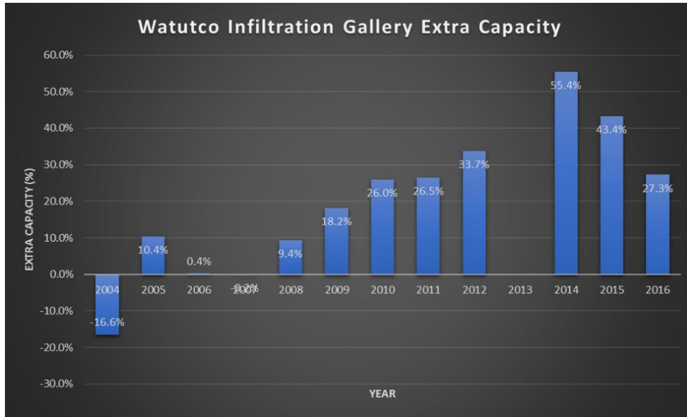
Figure 11 Watutco Infiltration Gallery Extra Capacity
