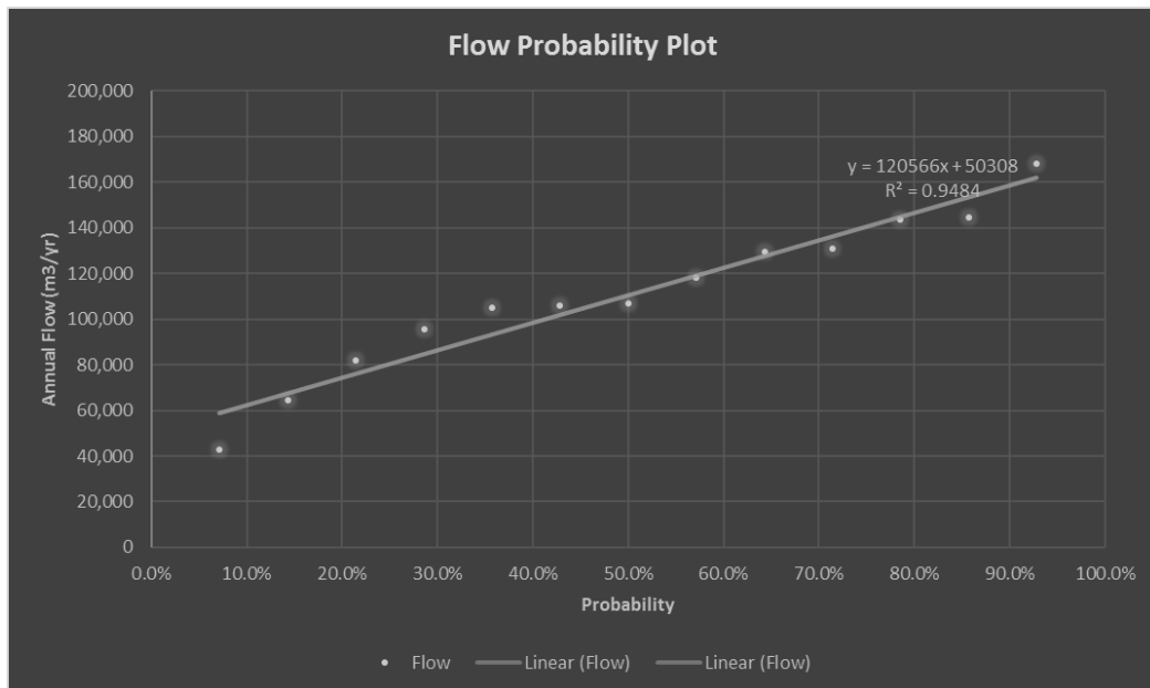
Figure 10 Flow Empirical Probability Plot
