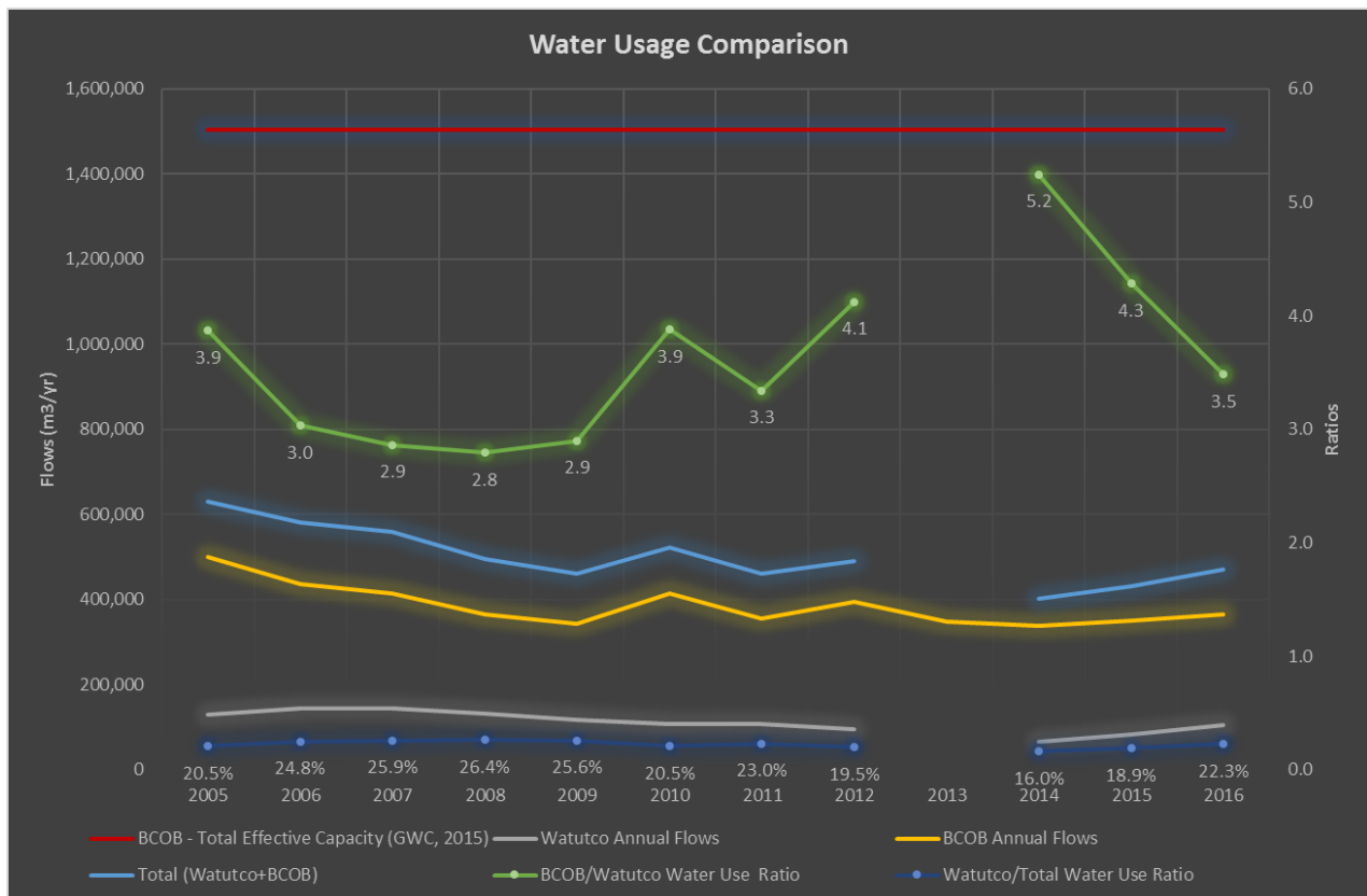
Figure 21 Water Usage Comparison
